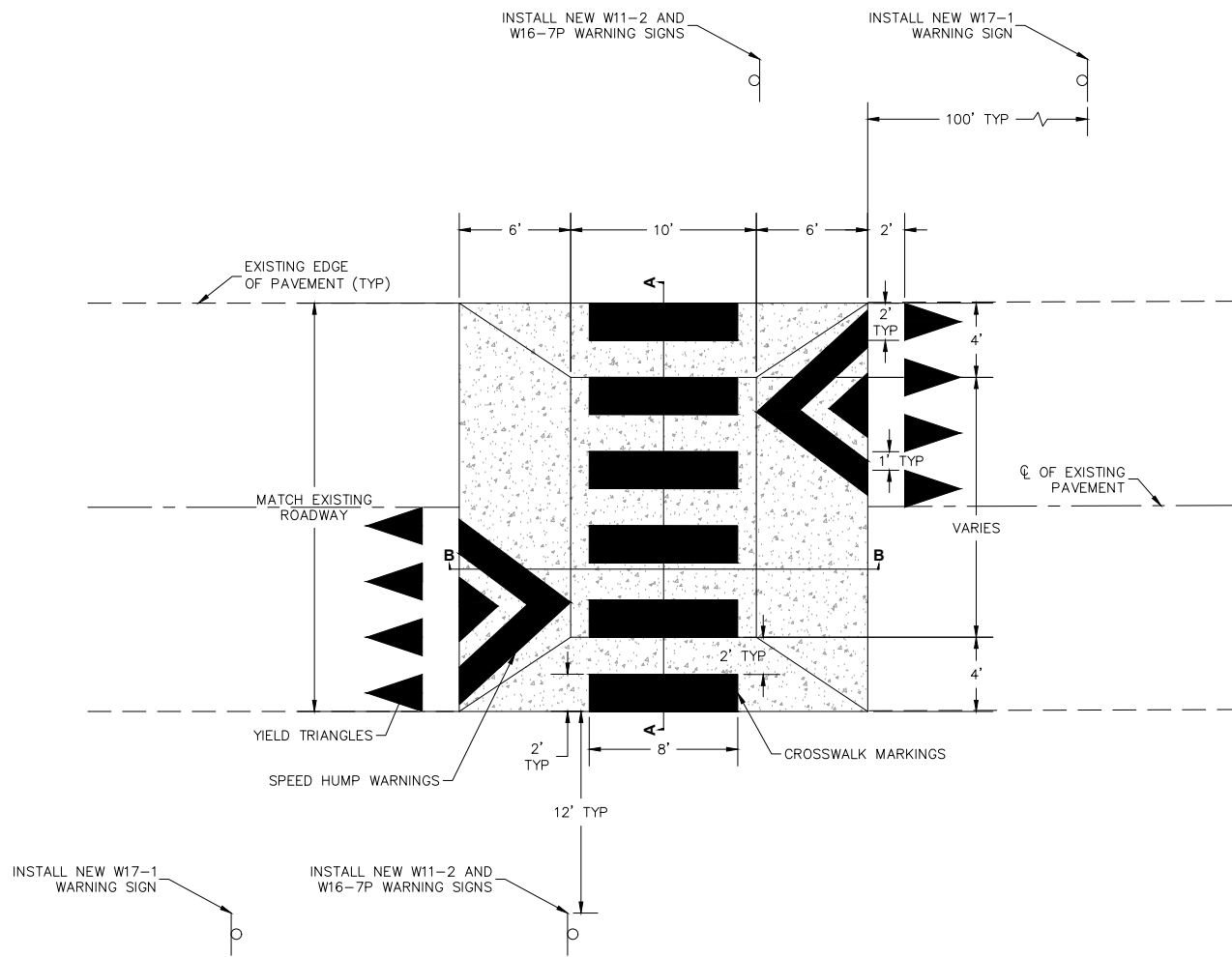
SPEED TABLE NO SCALE
