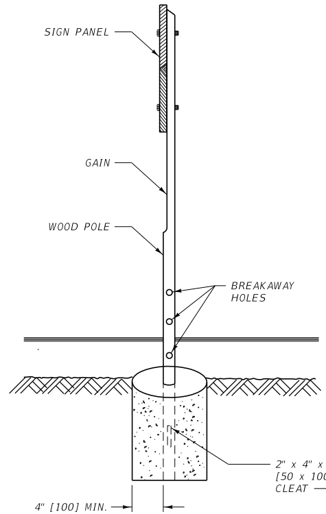
BREAKAWAY AND FOOTING DETAILS
