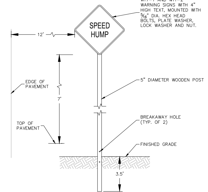
NOTE 5" DIAMETER WOOD POST TO BE INSTALLED PER MDT DETAIL DWG. NO. 619-20.
